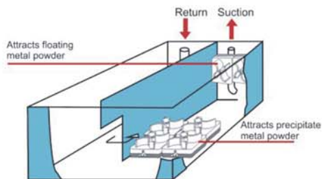
Coolant Tank
